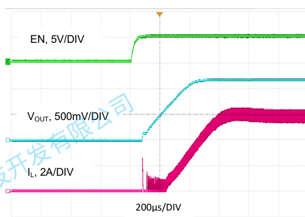
图 13. 启动波形, V_{OUT} = 1.2V , I_O = 6A
