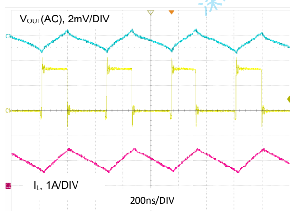
图 14. V_{OUT} = 1.2V , I_O = 1A , FPWM
