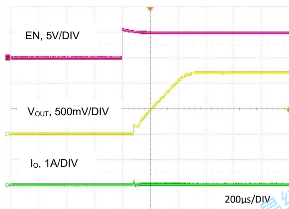
图 12. 启动波形, V OUT = 1.2V, I O = 10mA
