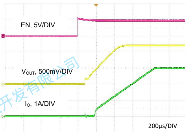
图 13. 启动波形, V OUT = 1.2V, I O = 3A
