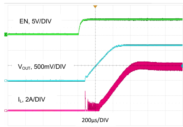
图 22. 启动波形, V_{OUT} = 1.2V , I_O = 6A
