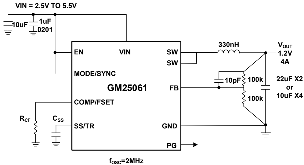
图 34. 2MHz, V IN =3.3V, V OUT =1.2V, I LOAD =4A
