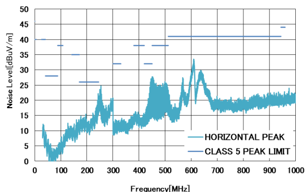
图 32. GM2506_DEMOZ CISPR25 Radiated Emission (Horizontal)
