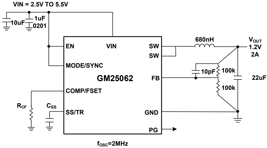
图 36. 2MHz, V IN =3.3V, V OUT =1.2V, I LOAD =2A
