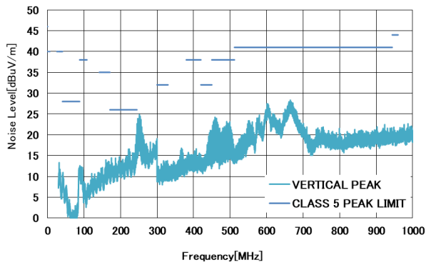
图 33. GM2506_DEMOZ CISPR25 Radiated Emission (Vertical)
