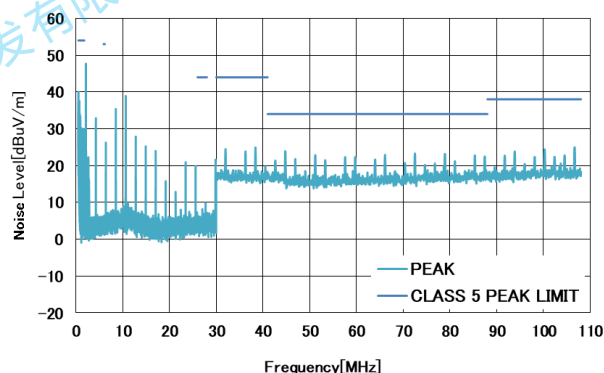
图 31. GM2506_DEMOZ CISPR25 Conducted Emission with Class 5 Peak Limits (Voltage Method)
