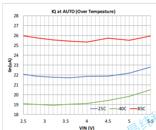
图17. I_Q vs V_{IN} 过热, Mode=Low, V_{OUT} = 1.8V
