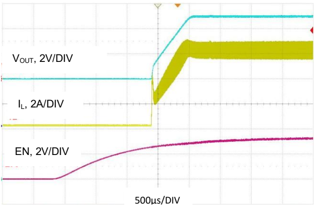
图 10. 启动波形, V_{OUT} = 5V , I_o = 6A
