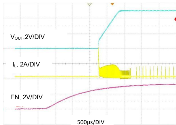
图 12. 启动波形, V_{OUT} = 5V , I_O = 10mA
