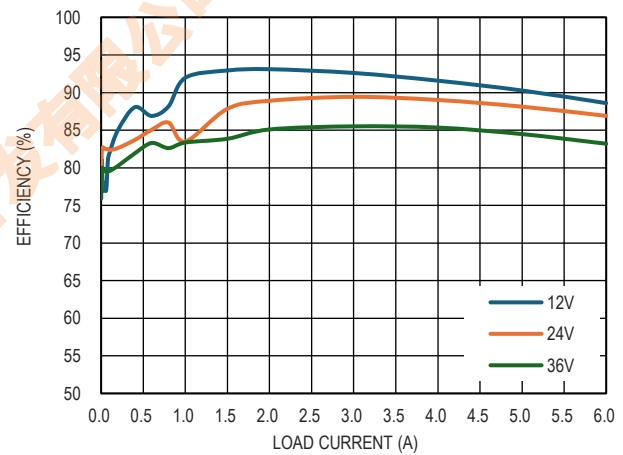
图 9. 效率曲线, V_{OUT} = 3.3V , L = 2.2uH , F_{SW} = 1MHz
