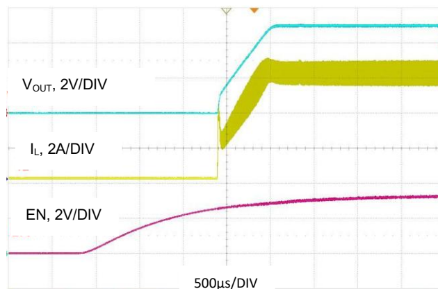
图 13. 启动波形, V_{OUT} = 5V , I_O = 6A
