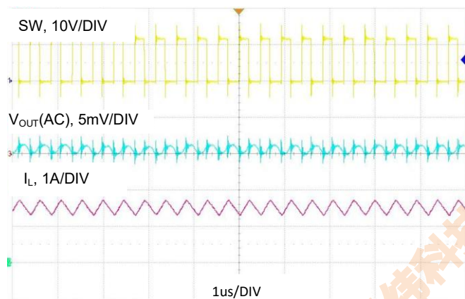
图 14. V_{OUT} = 5V , I_O = 3A , FPWM
