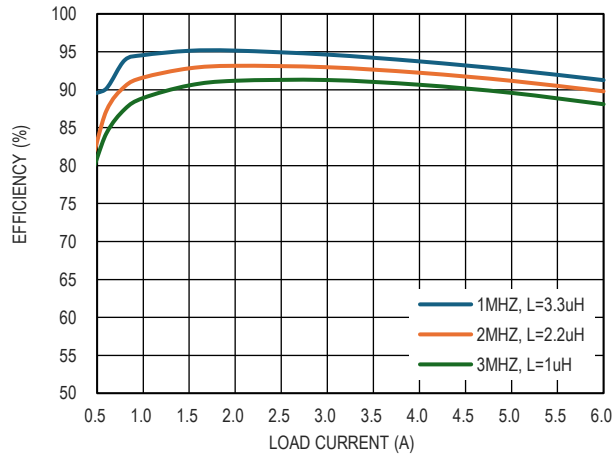
图 6. 效率曲线, V_{IN} = 12V , V_{OUT} = 5V
