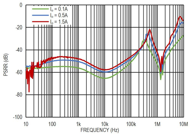
图 20. PSRR, V_{IN} = 5.3V , V_{OUT} = 5.0V
