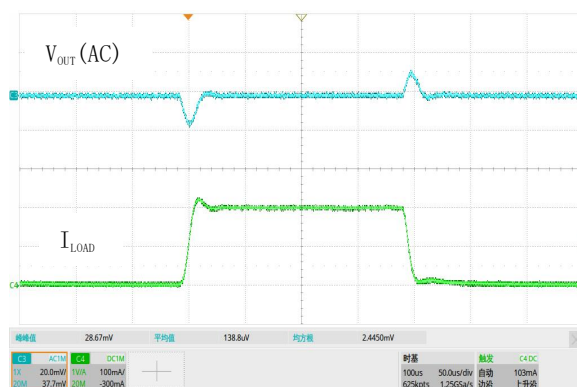
图 22. 负载瞬态响应, V_{IN}=4.3V , V_{OUT}=3.3V , I_{OUT}=1mA to 150mA
