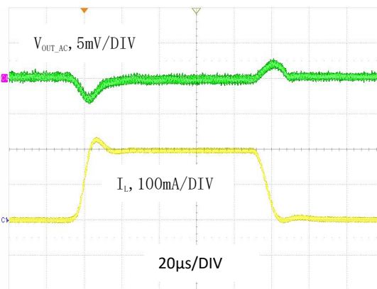
图 22. 负载瞬态响应, V_{IN}=4V , V_{OUT}=3.3V , I_{OUT}=1mA to 200mA
