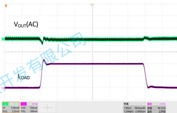
图 22. 负载瞬态响应, V_{IN}=4.3V , V_{OUT}=3.6V , I_{OUT}=5mA to 300mA
