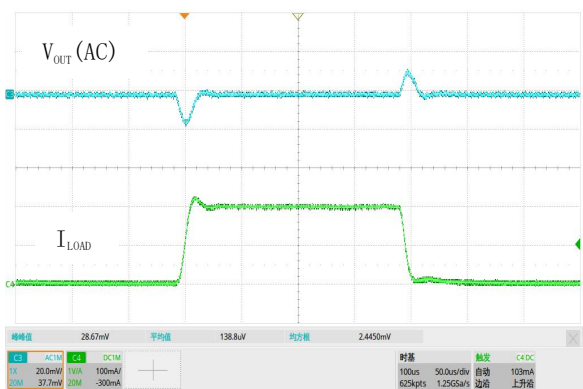
图 23. 负载瞬态响应, V_{IN}=4.3V , V_{OUT}=3.3V , I_{OUT}=1mA to 200mA
