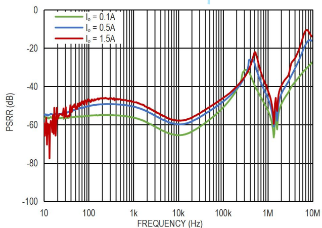
图 13. PSRR, V_{IN} = 5.3V , V_{OUT} = 5.0V
