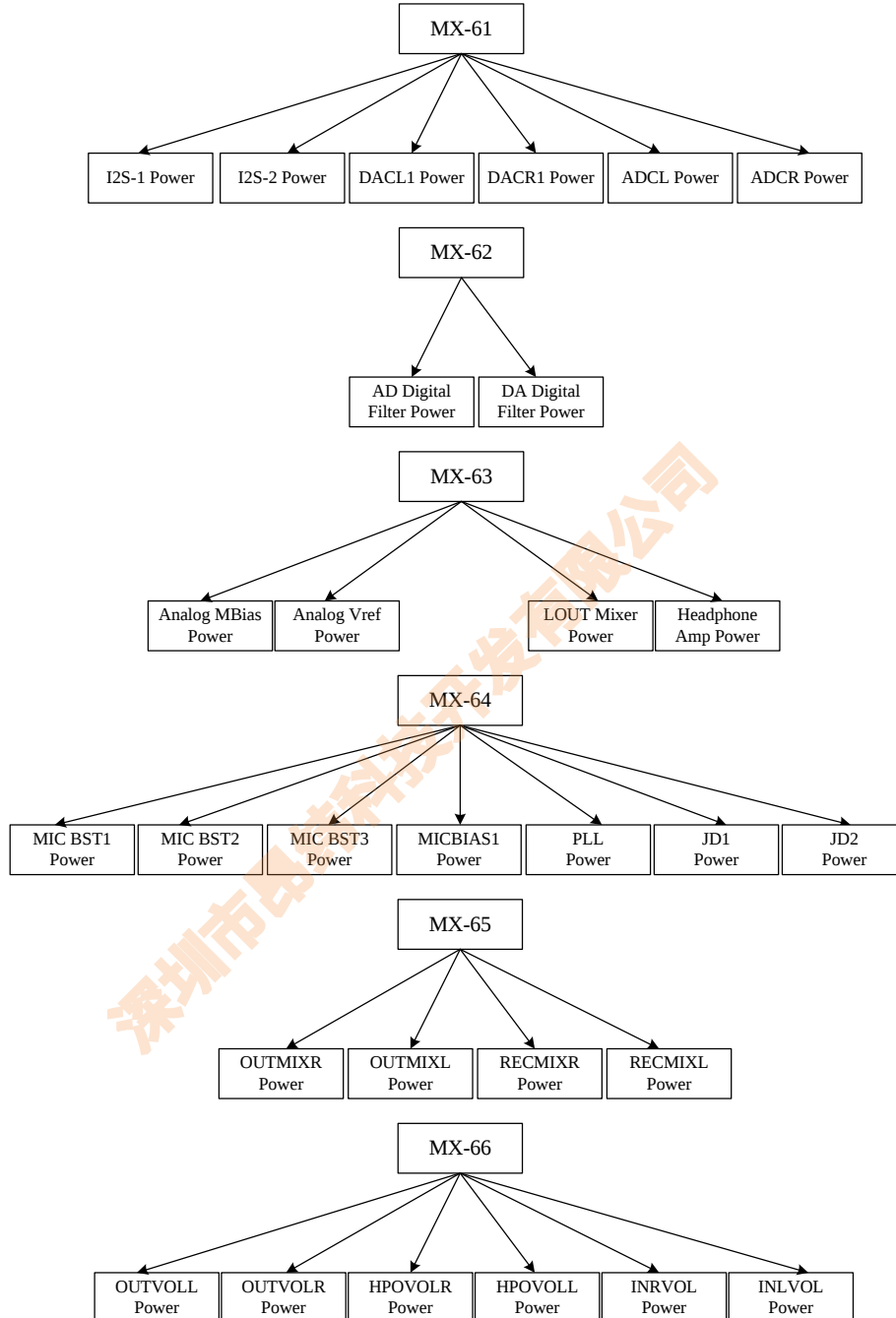
Figure 31. Power Management
