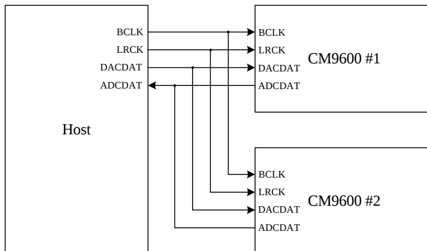
TDM Interface Application - 1
