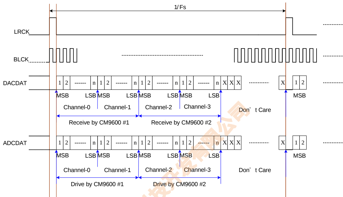
TDM Interface Application - 2
