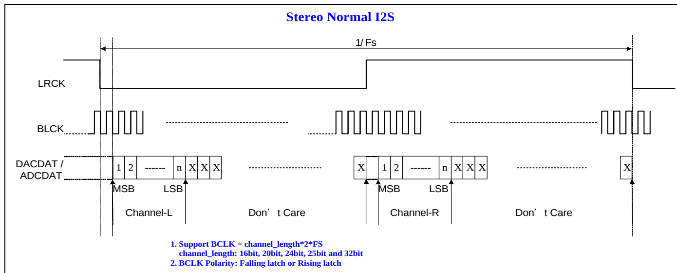
Figure 21. Stereo Normal I2S Data Format
