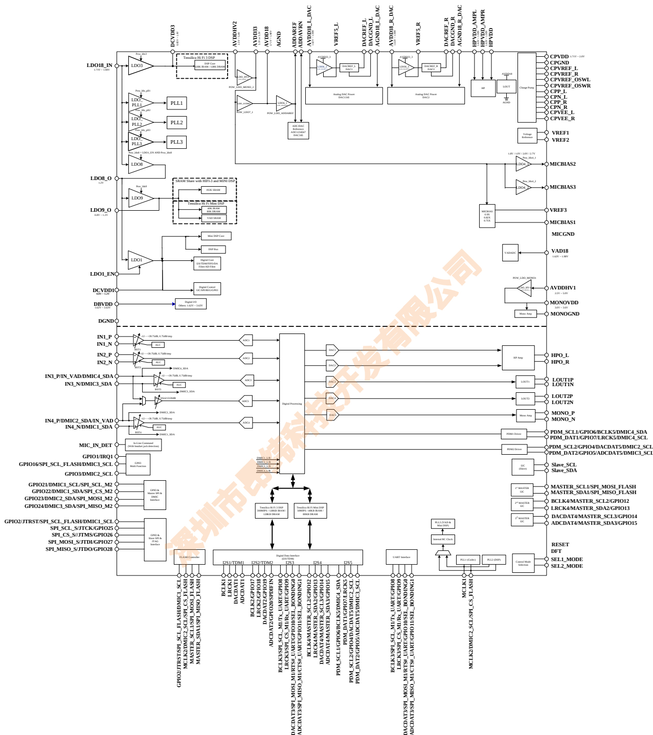
Figure 1. Function Block
