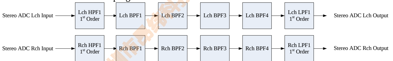
Figure 41. EQ Structure on the Record Path
