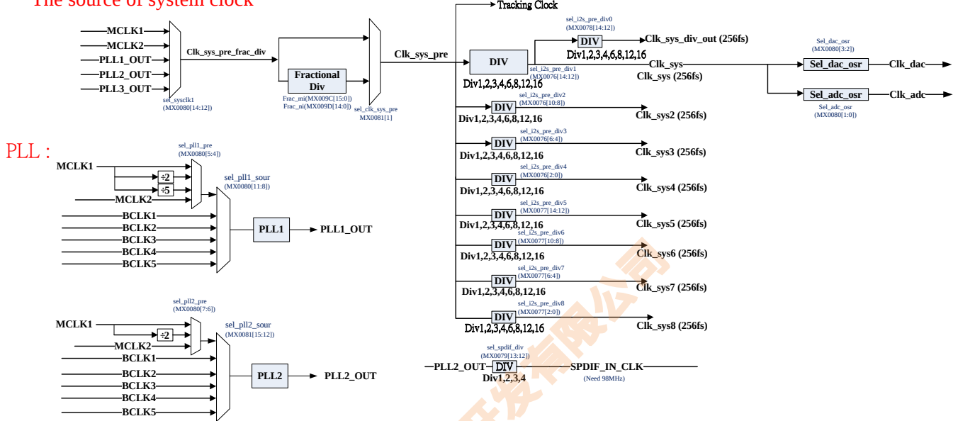
Figure 9. Codec System Clock Tree
