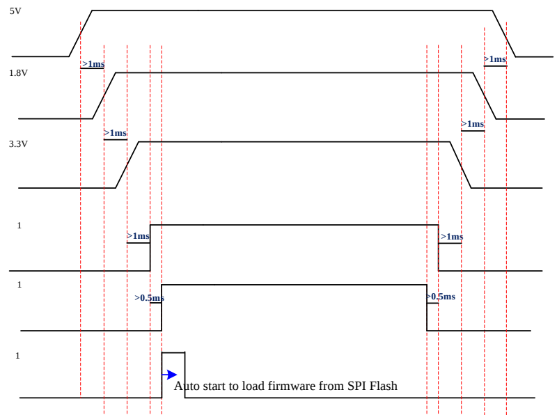
Figure 6. Power On/Off Timing when Normal Load Code by SPI Flash
