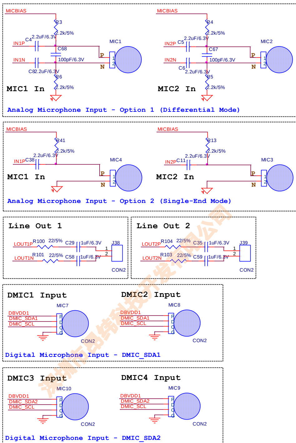
Figure 35. Application Circuit
