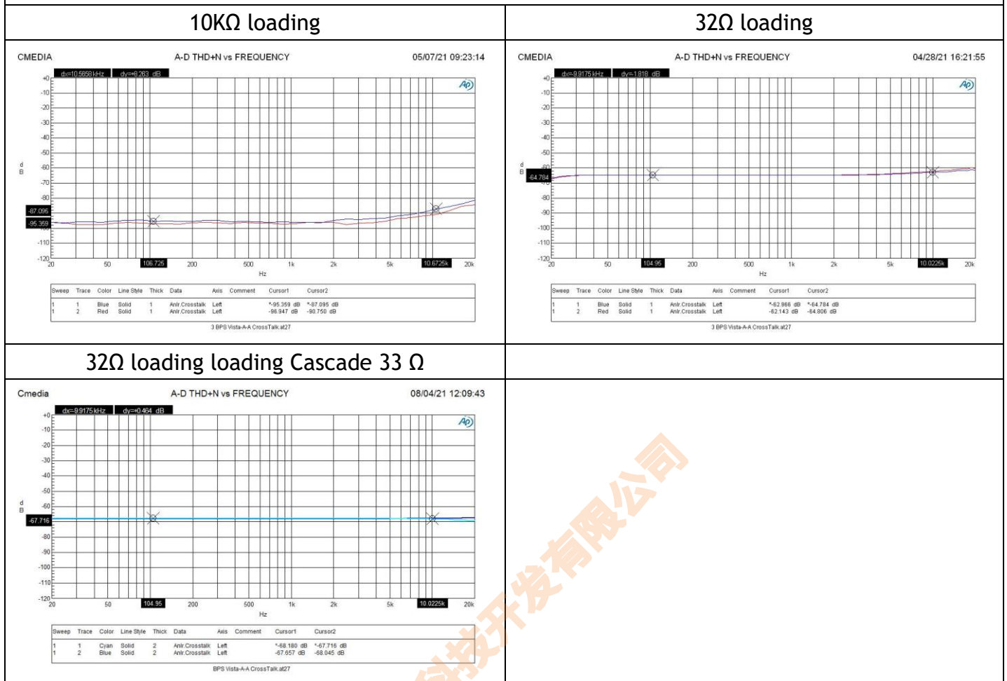
Figure 26 : A-A Cross-talk
