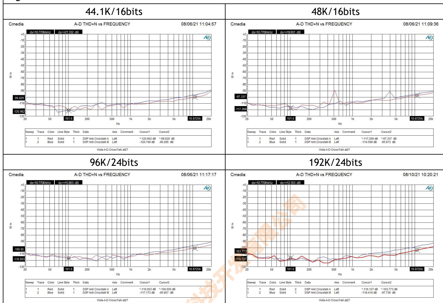
Figure 19 : ADC Cross-talk 0dB Gain
