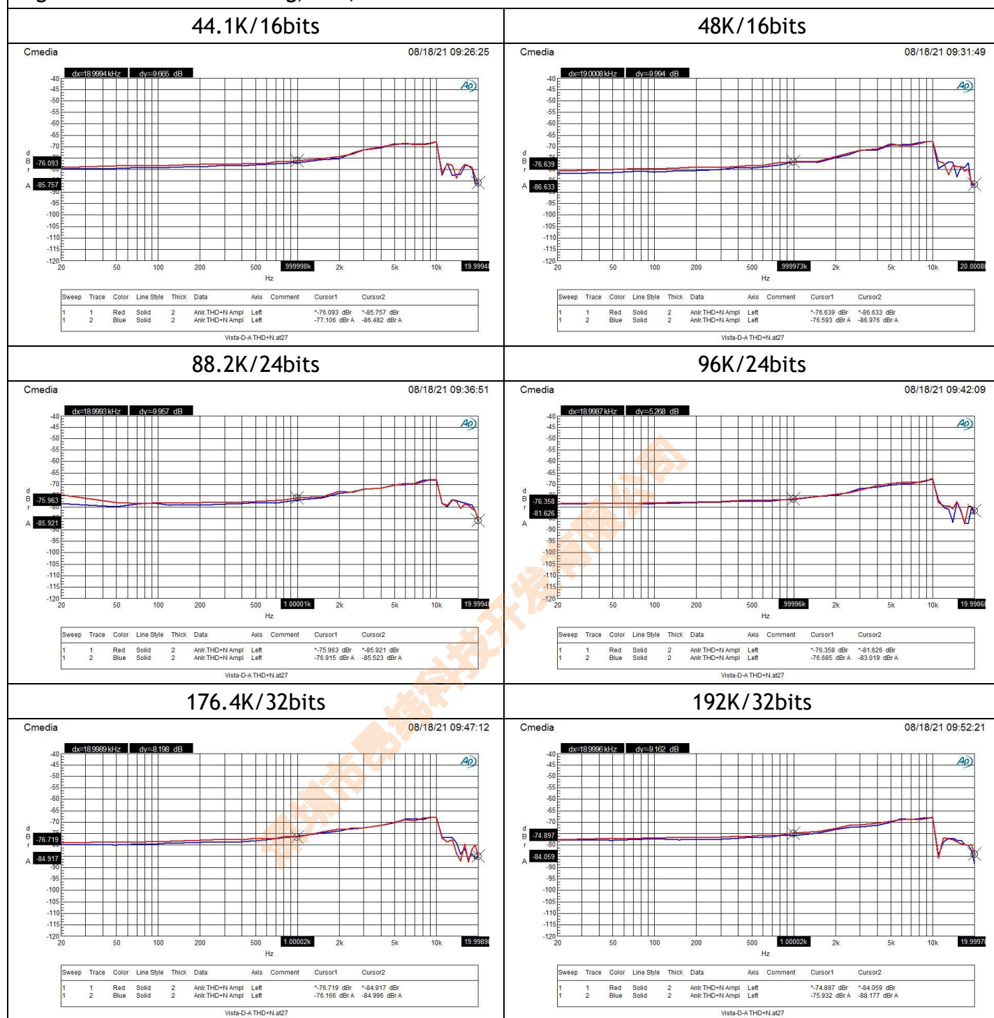
Figure 3 : DAC 32Ω loading, 0dB, THD+N
