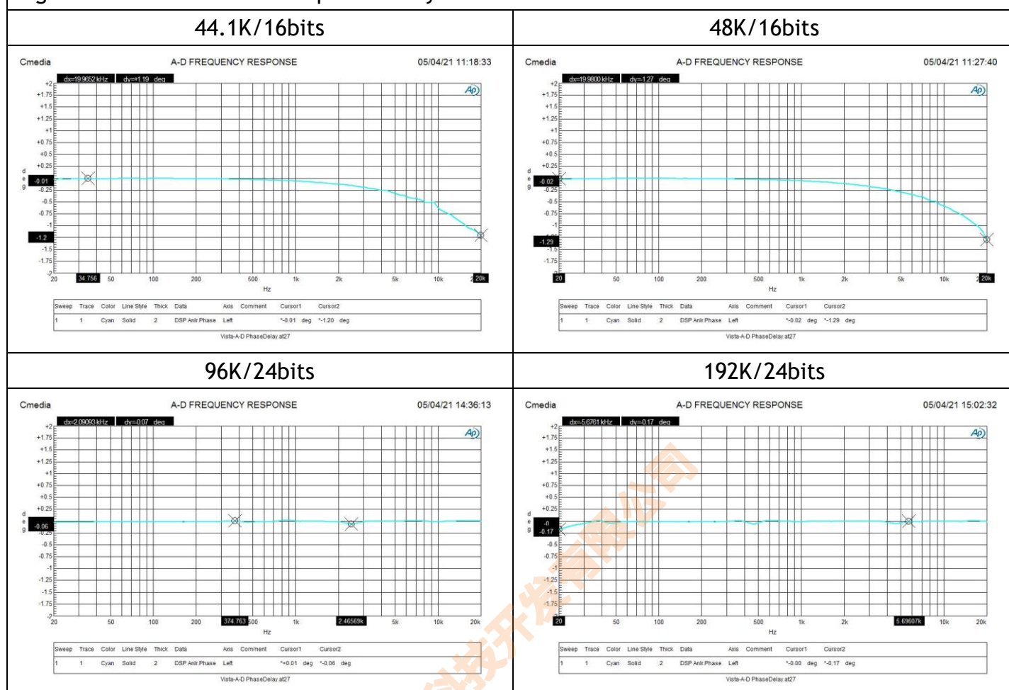
Figure 24 : ADC Interchannel phase delay 20dB Gain
