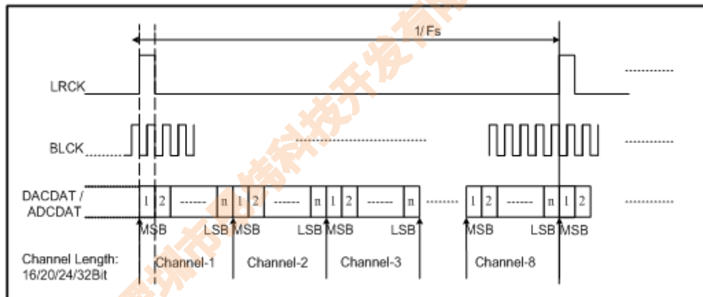
Fig. 7.6.2 TDM Mode 2 (BCLK POLARITY=0)
