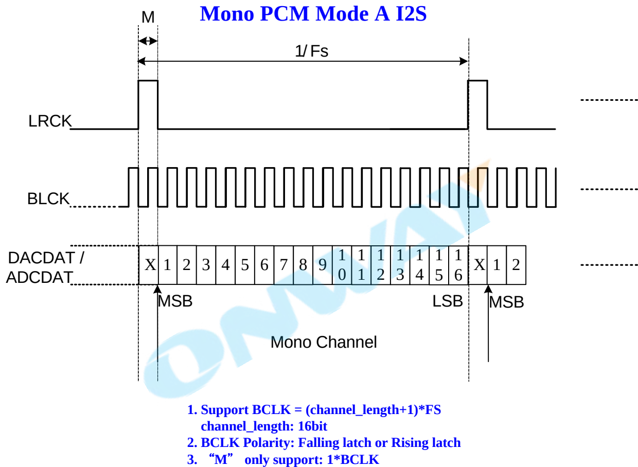
Figure 19. PCM/DSP Mono Data Mode A Format (bclk_polarity=0)
