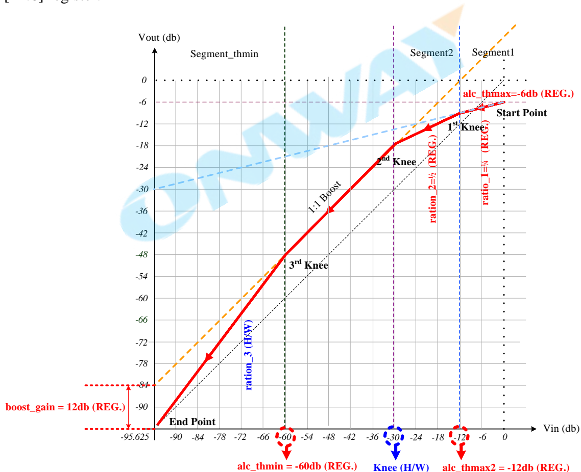
Figure 24. Playback DRC Output Curve
