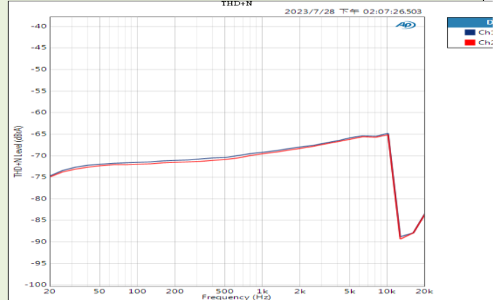
THD+N @ 32Ω loading Figure 17
