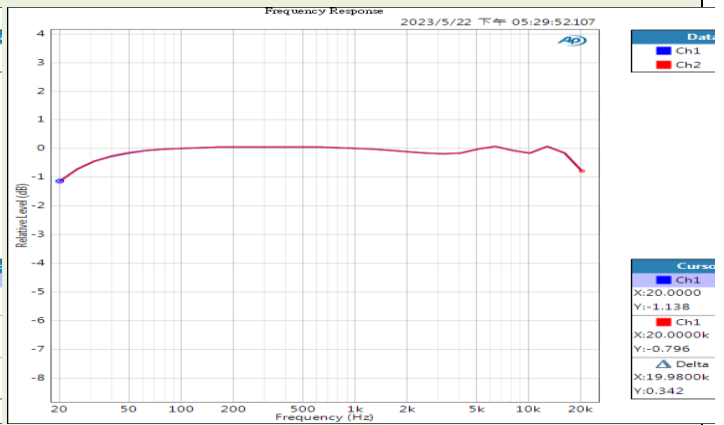
Frequency Response 20dB Gain Figure 15
