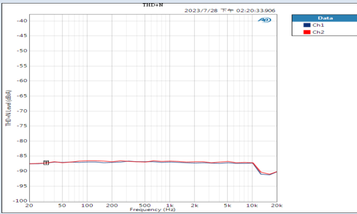
THD+N @ 10KΩ loading Figure 16
