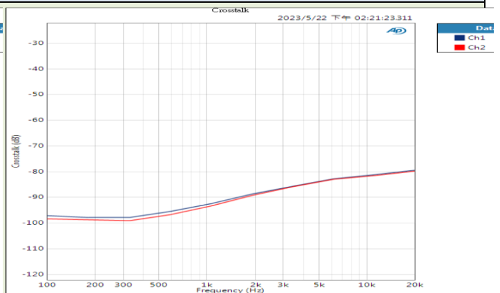
Cross-talk @ 32Ω with 33Ω cascade loading Figure 6
