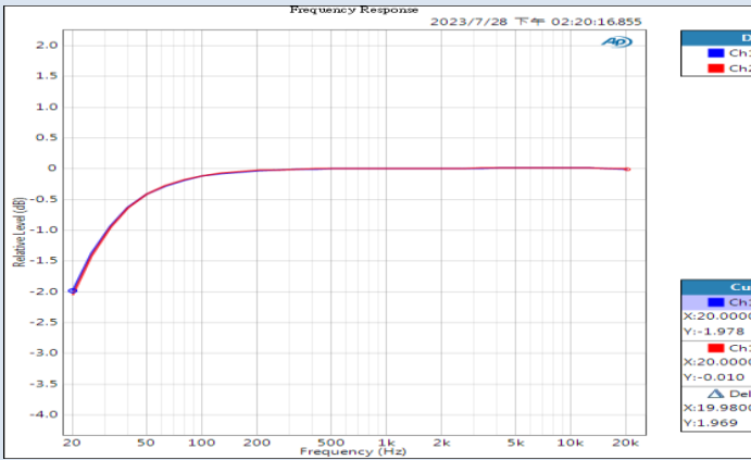
Frequency Response @ 10KΩ loading Figure 22
