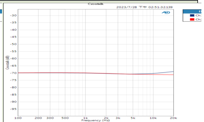
Cross-talk @ 32Ω with 33Ω cascade loading Figure 21
