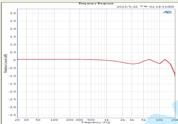
Frequency Response @ 32Ω with 33Ω cascade loading Figure 9
