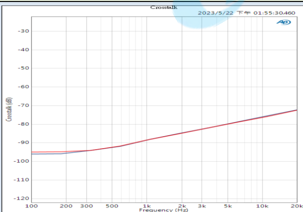
Cross-talk @ 32Ω loading Figure 5
