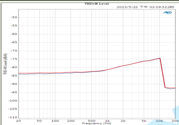
THD+N @ 32Ω with 33Ω cascade loading Figure 3
