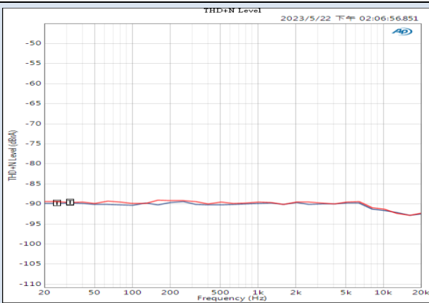
THD+N @ 10KΩ loading Figure 1
