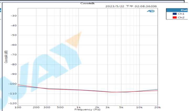
Cross-talk @ 10KΩ loading Figure 4
