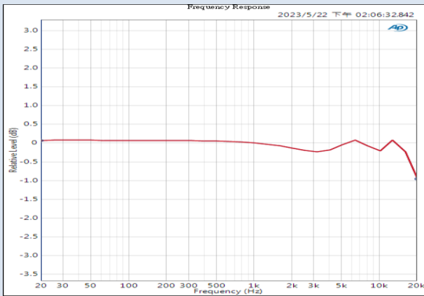
Frequency Response @ 10KΩ loading Figure 7
