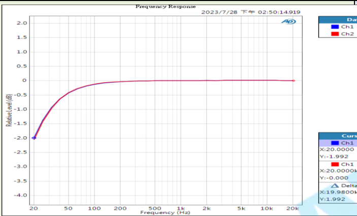
Frequency Response @ 32Ω with 33Ω cascade loading Figure 24
