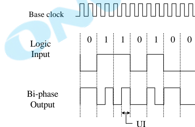
Fig. 6.3.2 S/PDIF biphasemark-code (BMC).
