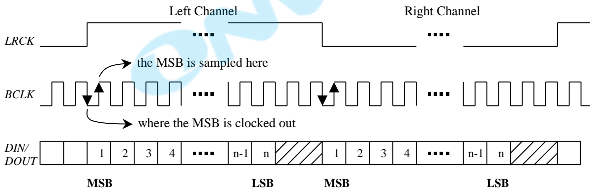
Fig. 6.6.2.1 LJ mode timing diagram of I2S interface.
