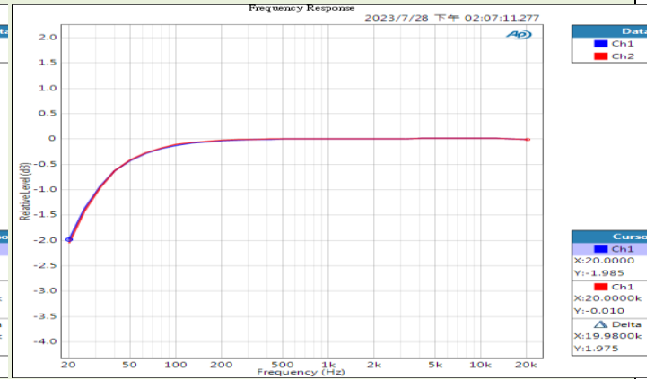
Frequency Response @ 32Ω loading Figure 23
