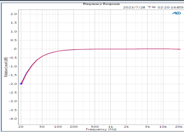
Frequency Response @ 10K \Omega loading Figure 22
