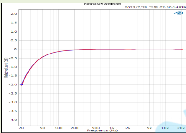
Frequency Response @ 32 \Omega with 33 \Omega cascade loading Figure 24
