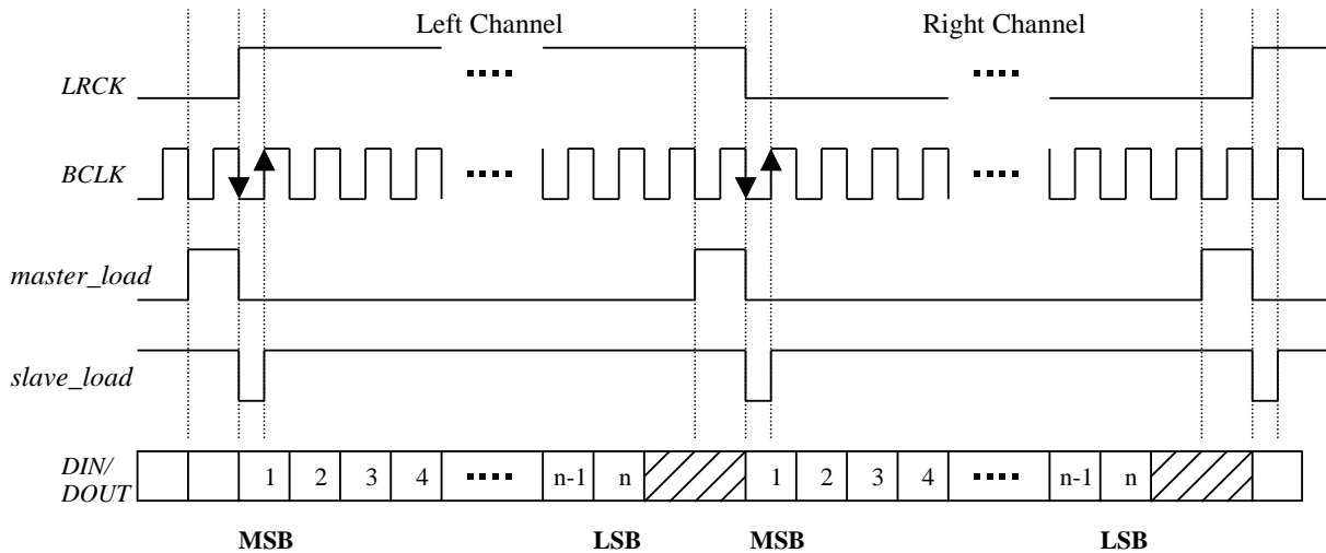
Fig. 6.6.5.1 The timing of load signal in I2S transmitter and receiver
