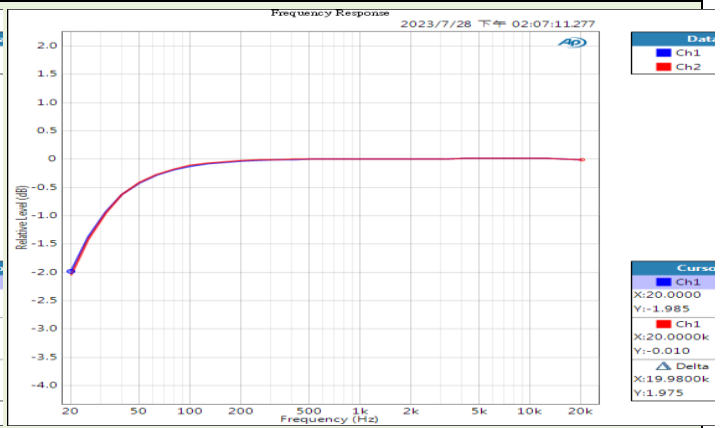
Frequency Response @ 32 \Omega loading Figure 23
